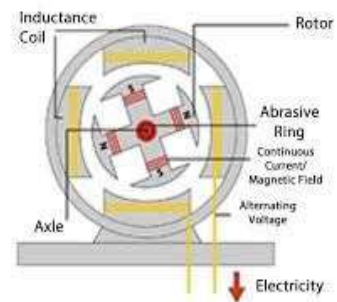
How a Magnetic Generator Works:
